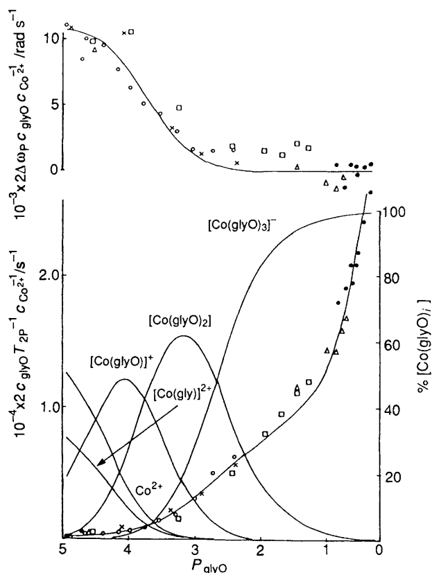
Figure 6. Normalized paramagnetic relaxation rate and shift data for the cobalt(II)-glycinate system measured on the \text{CH}_2 protons of the ligand, and the calculated curves together with the concentration distribution: c_{\text{H}}^0 = 1.5000 , c_{\text{glyO}}^0 = 1.5000 , c_{\text{Co}^{2+}} = 0.01054 ( \square ), 0.01054 ( \triangle ), 0.02007 ( \bullet ), 0.04214 ( \times ), 0.05144 mol \text{dm}^{-3} ( \circ )
