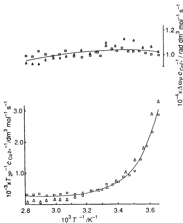
Figure 1. Temperature dependence of the paramagnetic relaxation rate and shift in an aqueous solution of \text{Co}^{2+} normalized for the total metal concentrations, together with the calculated curves; P_{\text{Co}^{2+}} = 5.912 \times 10^{-3} ( \Delta ) and 8.867 \times 10^{-3} ( \square )
