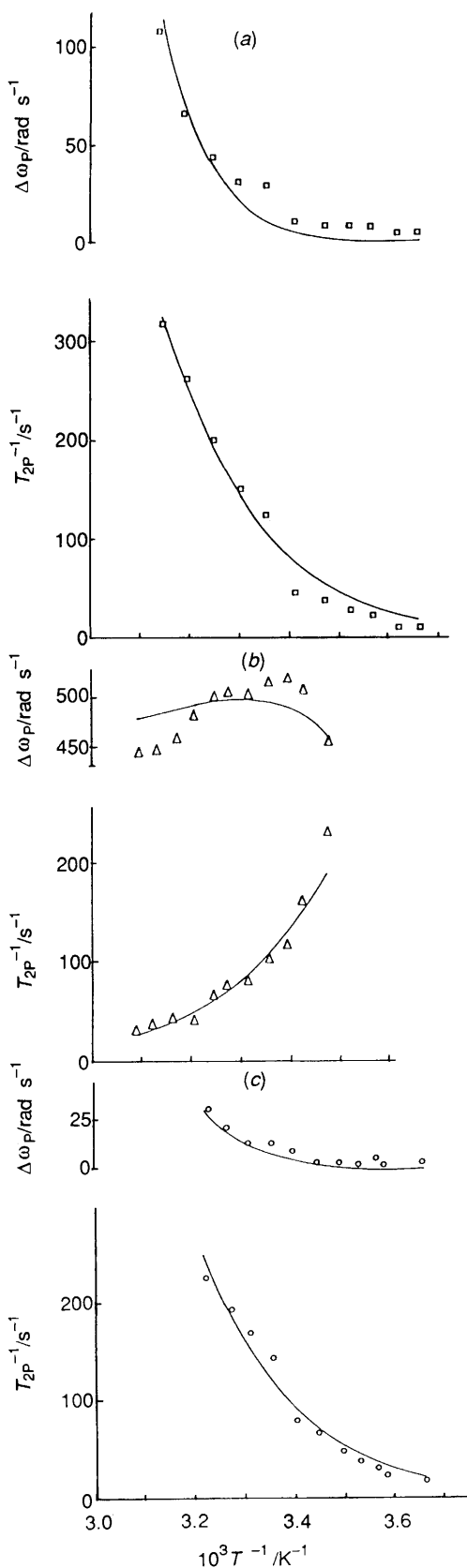
Figure 2. Temperature dependence of the paramagnetic relaxation rate and shift, together with the calculated curves, in solutions of (a) [\text{Co}(\text{en})_3]^{2+} ( P_{\text{Co}(\text{en})_3} = 3.412 \times 10^{-2} ), (b) relaxation rate and shift in the solutions of [\text{Co}(\text{mal})_2]^{2-} ( P_{\text{Co}(\text{mal})_2} = 1.133 \times 10^{-2} ), and (c) [\text{Co}(\text{glyO})_3]^- ( P_{\text{Co}(\text{glyO})_3} = 6.875 \times 10^{-2} )
