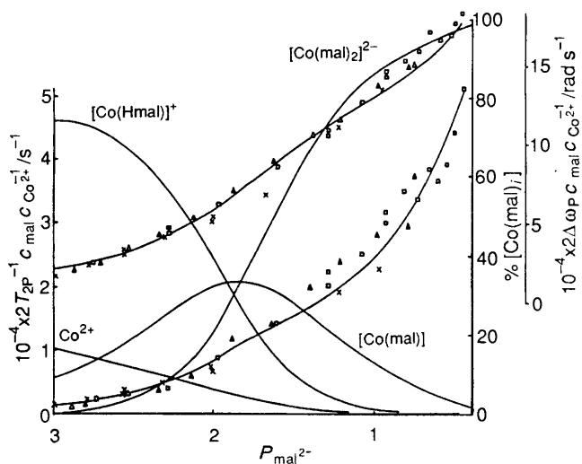
Figure 4. Normalized paramagnetic relaxation rate and shift data for the cobalt(II)-malonate system measured for the \text{CH}_2 protons of the ligand, and the calculated curves together with the concentration distribution: c_{\text{H}}^0 = 0.7231 , c_{\text{mal}}^0 = 0.5000 , c_{\text{Co}^{2+}}^0 = 0.00183 ( \square ), 0.00730 ( \times ); c_{\text{H}}^0 = 0.5511 , c_{\text{mal}}^0 = 0.4000 , c_{\text{Co}^{2+}}^0 = 0.00365 ( \Delta ), 0.01825 \text{ mol dm}^{-3} ( \circ )
