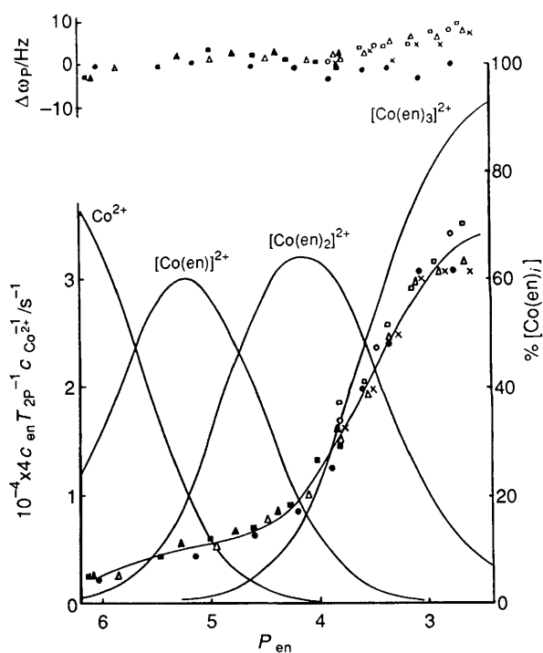
Figure 3. Normalized paramagnetic relaxation rate data for the cobalt(II)-ethylenediamine system detected for the \text{CH}_2 protons of the ligand, and the calculated curve together with the concentration distribution: c_{\text{H}}^0 = 1.0466 , c_{\text{en}}^0 = 0.5137 , c_{\text{Co}^{2+}}^0 = 0.00547 ( \times ), 0.00730 ( \Delta ), 0.00912 ( \square ), 0.01368 ( \circ ), 0.01825 ( \blacktriangle ), 0.02737 ( \blacksquare ); c_{\text{H}}^0 = 1.1266 , c_{\text{en}}^0 = 0.5089 , c_{\text{Co}^{2+}}^0 = 0.01825 \text{ mol dm}^{-3} ( \bullet )
