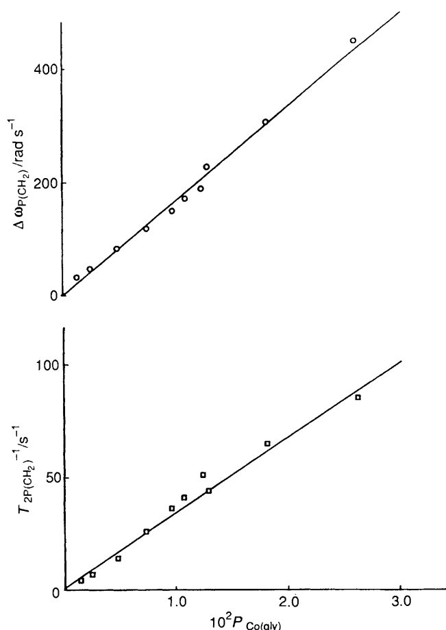
Figure 5. Paramagnetic relaxation effect of [\text{Co}(\text{gly})]^{2+} detected for the \text{CH}_2 protons of the ligand (pH 3.25)
